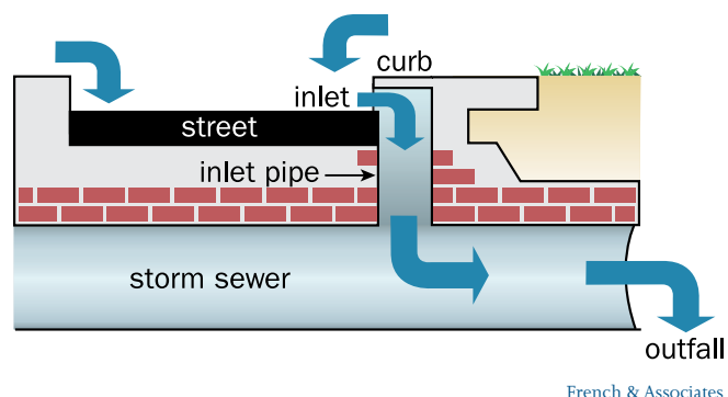
Storm sewer terminology.
