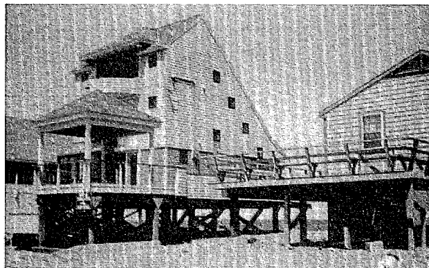
Residences are typically elevated on pressure-treated, cross-braced wood piles. One local contractor constructs over 25 residential elevation projects a year.
